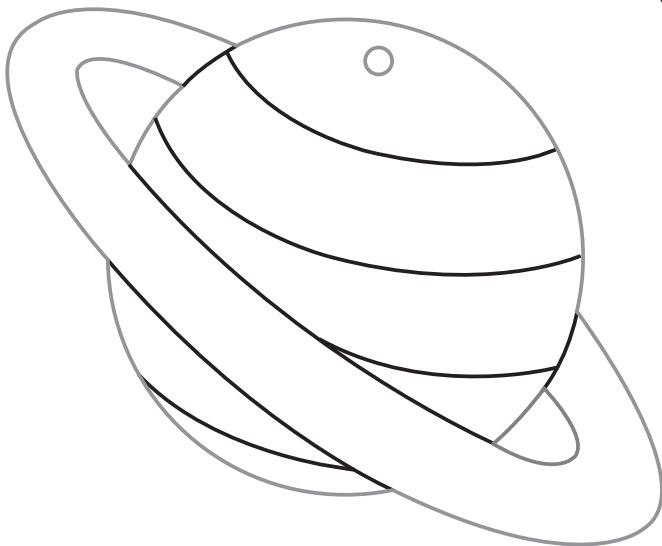
Saturn
