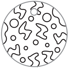
Mercury
